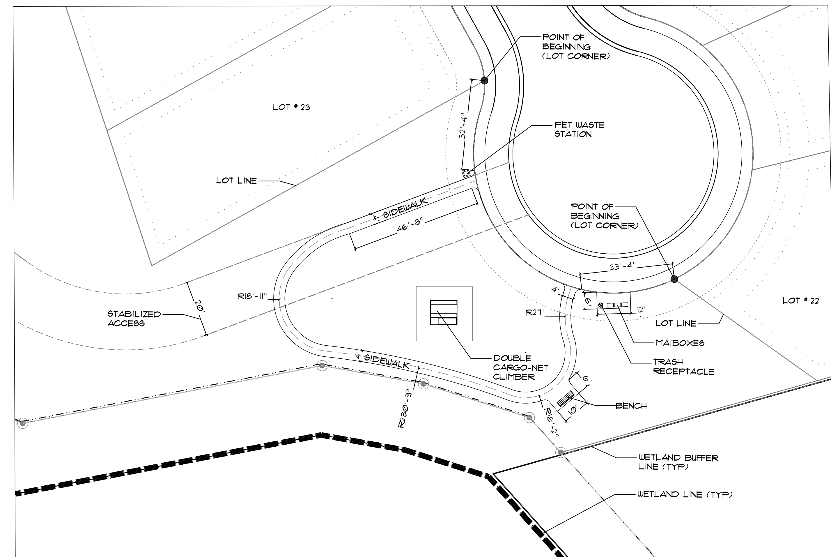
NEIGHBORHOOD PARK 'B' SCALE: 1"=20'
